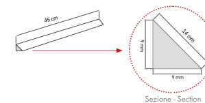
Dettaglio quarter round - Quarter round detail
