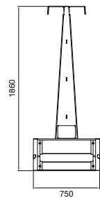
Zinc-plated sheet A-frame
