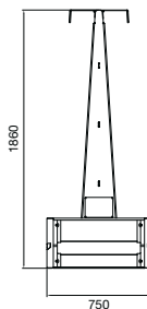
Zinc-plated sheet A-frame
